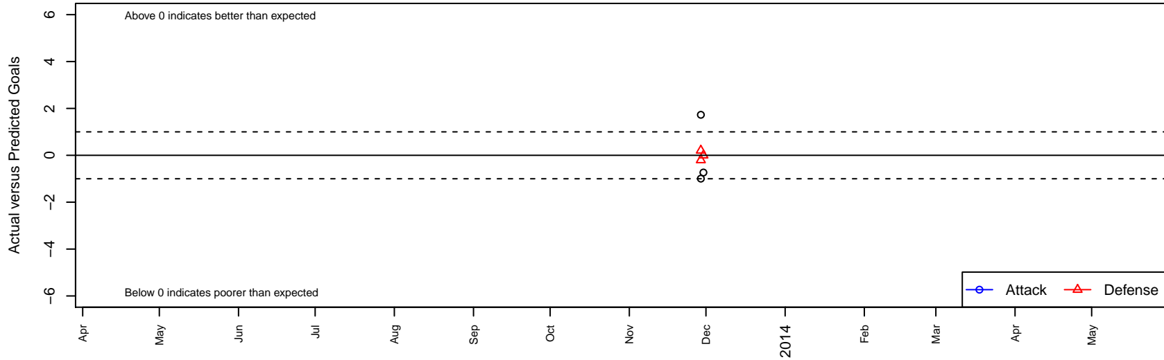
CAS Pumas UNAM B02 Dots are actual minus expected GF (blue circles) and GA (red triangles). Blue line is smoothed change in attack strength. Red is smoothed change in defense strength.
